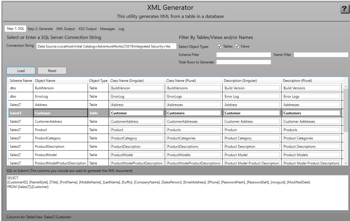
Figure 14: Step 1: XML Generator SQL Tab.
