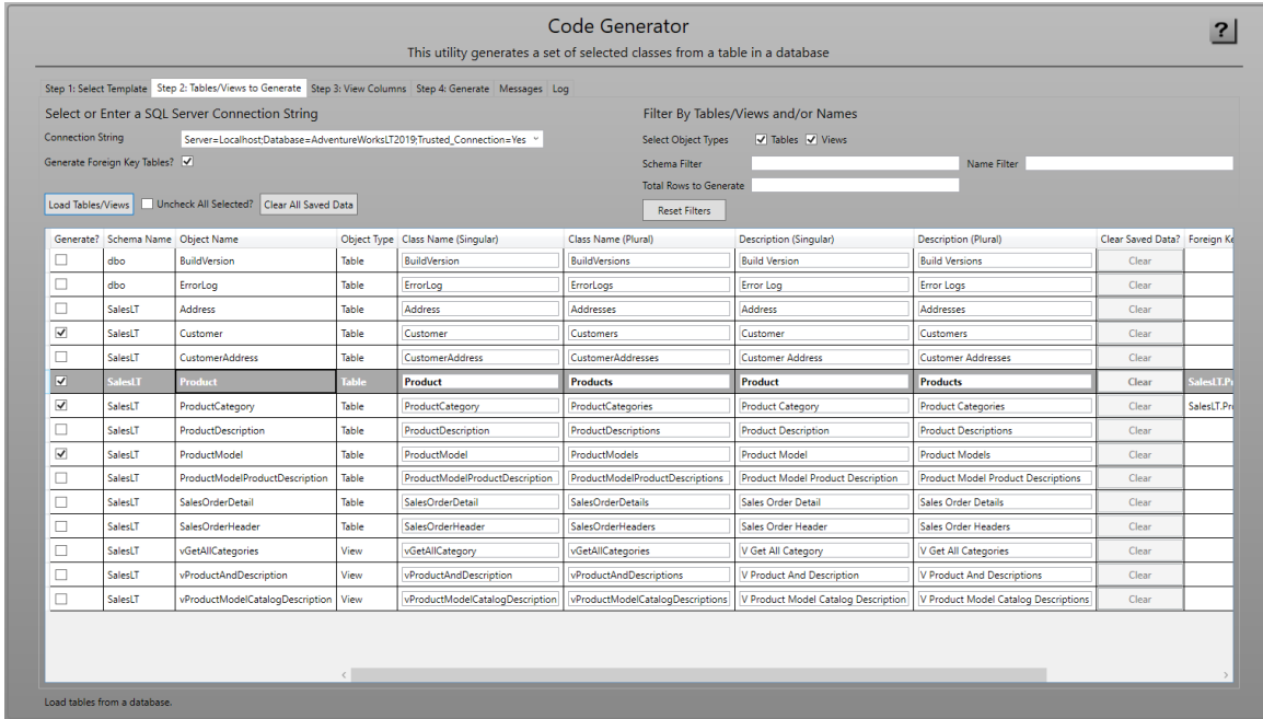
Figure 19: Step 2: Code Generator Tables/Views to Generate Tab.
