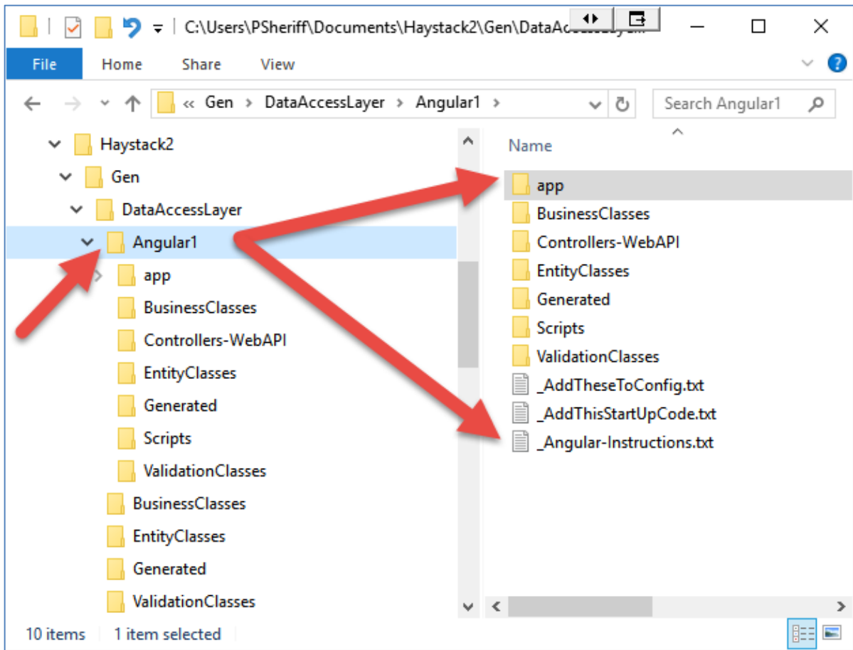
Figure 10: Copy all folders from the WebAPI folder into your Visual Studio project
